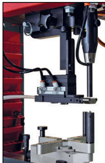
Multi-shuttle tooling platform for nuts studs and standoffs.
