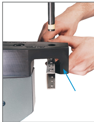
Bottom Mount Reverse Flange Anvil Holder.
